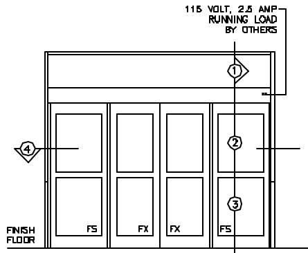
EXTERIOR ELEVATION
